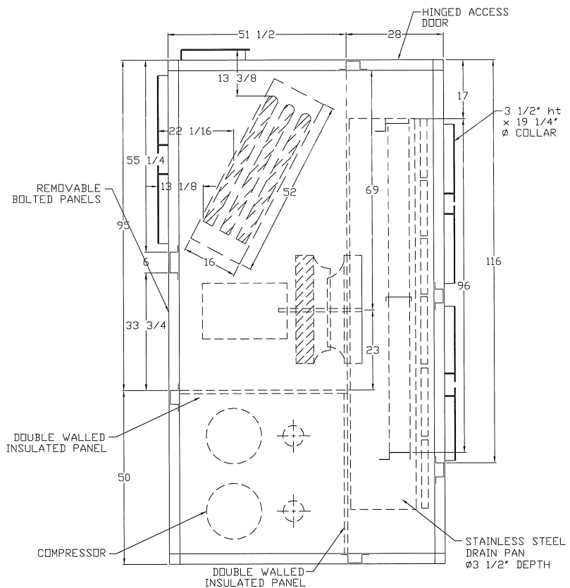
PLAN VIEW OF EVAP. BLOWER SECTION ONLY
